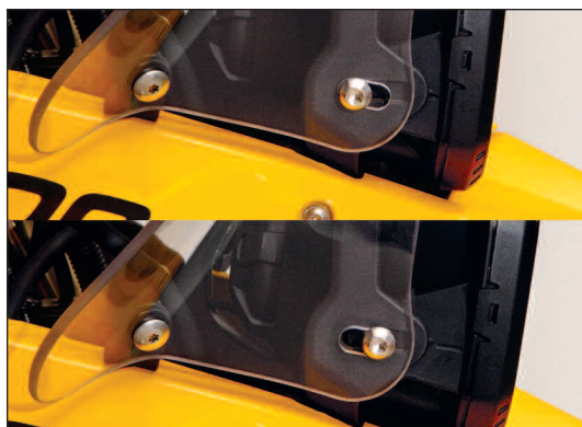
These VStream Windscreens use the headlight as an additional mounting point while maintaining complete headlight adjustability.
